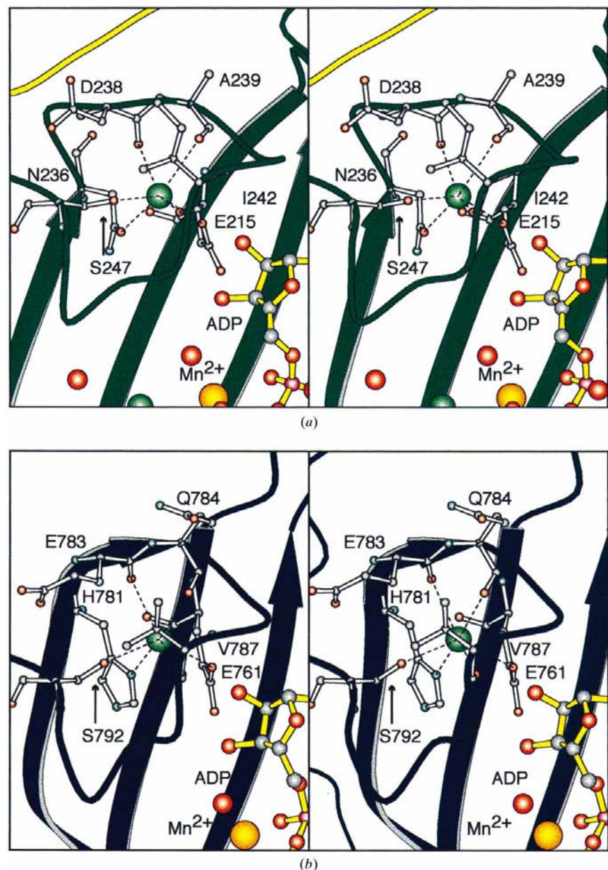
Figure 8 The 'K-loops' associated with the two synthetase units of the CPS large subunit. The potassium ion located in the carboxyphosphate synthetic component is shown in (a). As indicated by the large green sphere, this cation is surrounded by oxygen ligands in an octahedral coordination sphere. Note the close proximity of the 2'- and 3'-hydroxyl groups of the ADP ribose to the potassium ion. The potassium ion located in the carbamoyl phosphate synthetic component is shown in (b). Ordered water molecules are depicted as red spheres.
