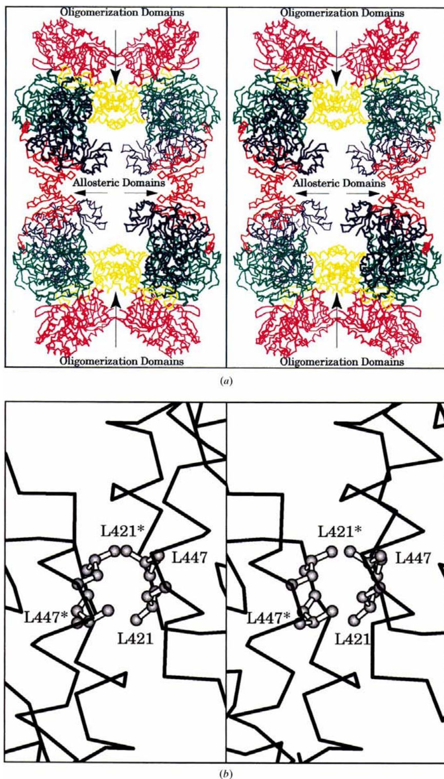
Figure 9 \alpha -Carbon trace of the entire CPS ( \alpha,\beta ) 4 -tetramer. (a) The oligomerization domains are as indicated. A close-up view of the subunit:subunit interface formed by these domains is given in (b). As indicated, the primary hydrophobic interactions occur between Leu421 and Leu447 and their symmetry-related partners, Leu421* and Leu447*.
